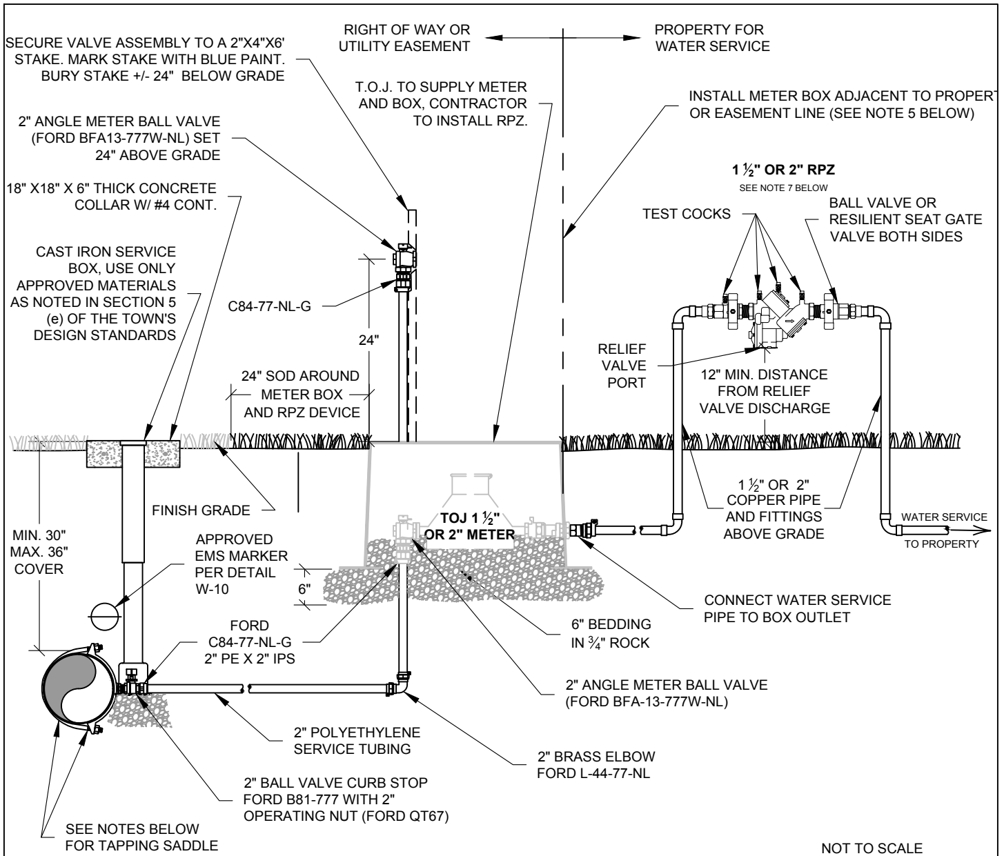
TYPICAL SAME-SIDE SERVICE TAP (SEE DETAIL W-23 FOR ROAD CROSSING REQUIREMENTS)
