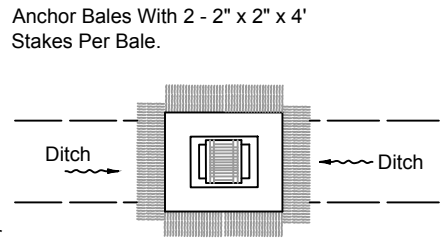
DITCH BOTTOM INLET
