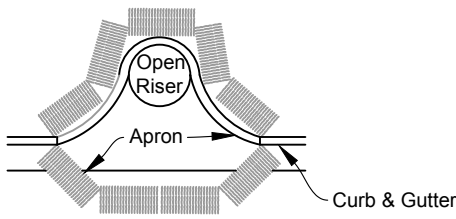
PARTIAL INLET
