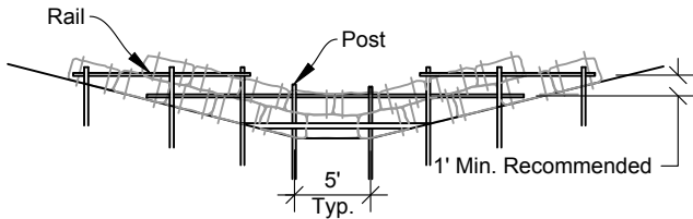
ELEVATION TYPE II
